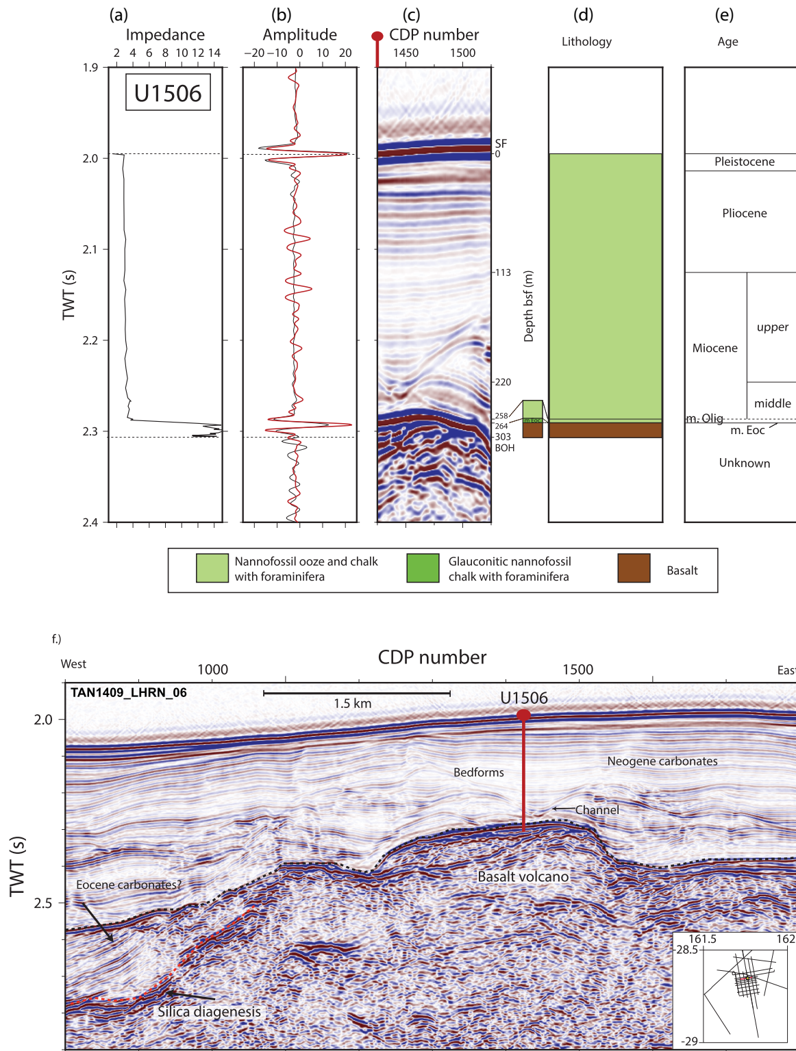
Figure 3. Borehole ties to seismic and timing of tectonic events at Site U1506. (a) Impedance (velocity × density) plotted against TWT for the borehole using the data shown in Fig. 2. This impedance model is used to produce the synthetic seismic trace (red) in (b). (b) Synthetic solution for the borehole (in TWT) plotted against real seismic trace data extracted from the borehole site. (c) Sample of seismic data near the borehole showing the seismic characteristics at the borehole site (right axis is marked as depth bsf in metres). Red marker at top of plot shows location of the borehole. BOH is bottom of hole. SF is seafloor. (d) Lithologic interpretation. (e) Geological timescale interpreted from the fossil assemblage and palaeomagnetic data of the core. (f) Seismic section showing geological structure near the borehole. Red marker shows the location and depth of the borehole. Labels indicate interpreted stratigraphic and tectonic horizons. Inset shows the site survey and regional seismic lines used to determine structure in vicinity of the borehole. Red line shows the location of the seismic data shown in main figure. Yellow star is the borehole site.
