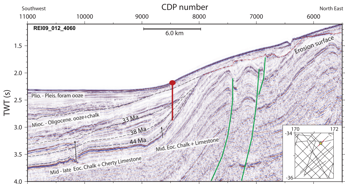
Figure 5. Borehole ties to seismic and timing of tectonic events at Site U1508. See the caption for Fig. 3 for further explanation. Green lines are fault traces.
