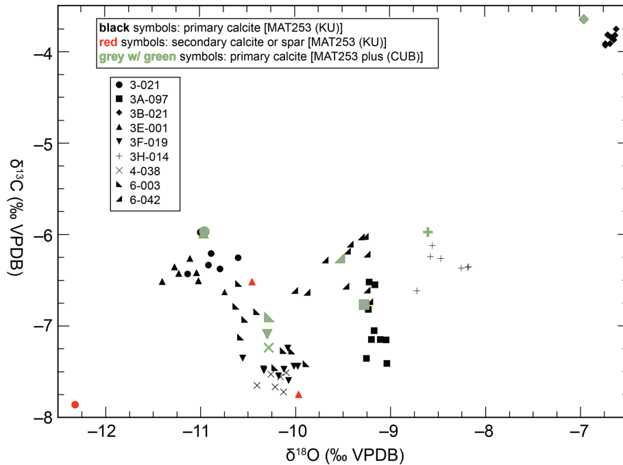
Figure 4. Carbonate \delta^{13}\text{C} and \delta^{18}\text{O} for White Pagoda samples. Black symbols represent drill spot measurements of inferred primary calcite and red symbols represent drill spot measurements of inferred secondary calcite (measured at KU). Gray with green symbols represent mean \delta^{13}\text{C} and \delta^{18}\text{O} measured on larger inferred primary calcite samples at CUB.
