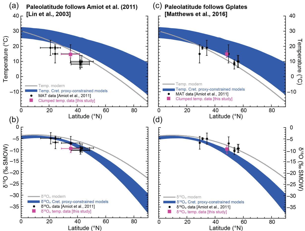
Figure 7. Northern Hemisphere latitudinal gradients of temperature and meteoric water \delta^{18}\text{O} for the mid-Cretaceous (Barremian–Albian). Our mean record data (pink) and the data of Amiot et al. (2011) (black) are plotted with a range in modeled gradients of Cretaceous climate as a function of latitude (blue shaded area) compiled in Suarez et al. (2011a). Details on models included in this range are in the main text. Modern temperature and meteoric water \delta^{18}\text{O} (gray lines) are plotted following Rozanski et al. (1993). The 1\sigma uncertainty is included for all data. Two paleolatitude reconstructions are considered: Lin et al. (2003) (a, b) and Matthews et al. (2016) (c, d). Uncertainty in latitude is included in panels (a) and (b); reconstructions of Matthews et al. (2016) do not provide uncertainty.
