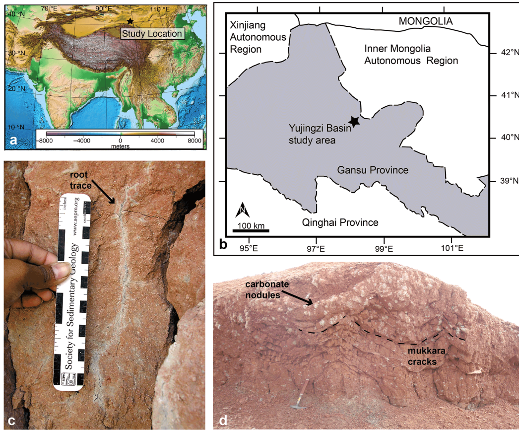
Figure 1. Approximate location of sampled sections with respect to regional topography (a; Amante and Eakins, 2009) and geography (b). Outcrop images of carbonate nodule bearing Vertisol section typical of the composite study section (c, d). Root traces, muklara cracks, ped structure and coloration (Retallack, 1997) are all indicative of Vertisols.
