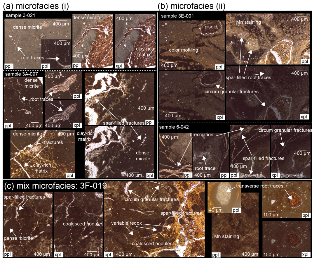
Figure 2. Annotated photomicrographs from select carbonate nodules of the White Pagoda Site. Samples are split into two microfacies (a, b) with sample 3F-019 appearing to be a mixture of the two microfacies (c).
