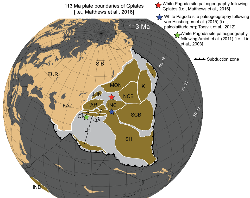
Figure 6. Paleogeographic reconstruction of plate boundaries at ca. 113 Ma (Matthews et al., 2016) using the Gplates software. Approximate location of the White Pagoda site following Matthews et al. (2016) is plotted in red. Additional paleogeographic reconstructions are also plotted for comparison (Lin et al., 2003; Torsvik et al., 2012), although these paleolocations are inconsistent with plate boundary reconstructions shown here (i.e., do not follow Matthews et al., 2016). The Aptian–Albian paleolatitude using the Gplates software is more consistent with the cooler temperatures indicated by clumped isotope paleothermometry.
